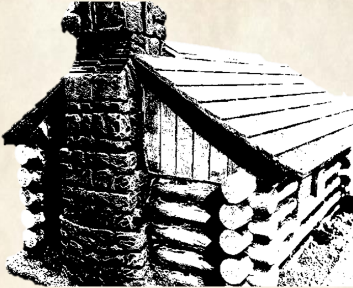
Figure 16. Basic square-shaped log cabin fireplace
