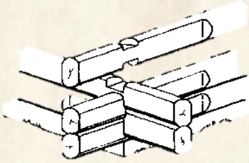
Figure 19. Lock notching
