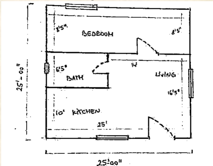
Figure 12. Log cabin
