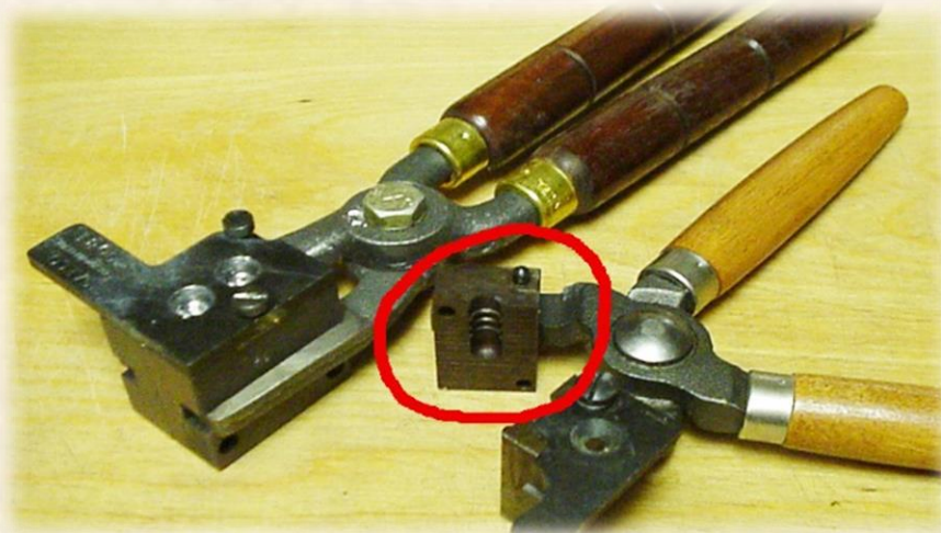
(Two bullet molds. The single cavity mold is open and empty. The double cavity mold is closed and contains two bullets. Photo Credits: Thewellman)
